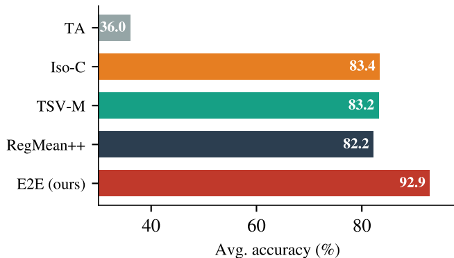
ViT-L/14 (20 tasks)
