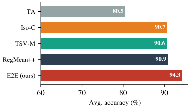
ViT-L/14 (8 tasks)
